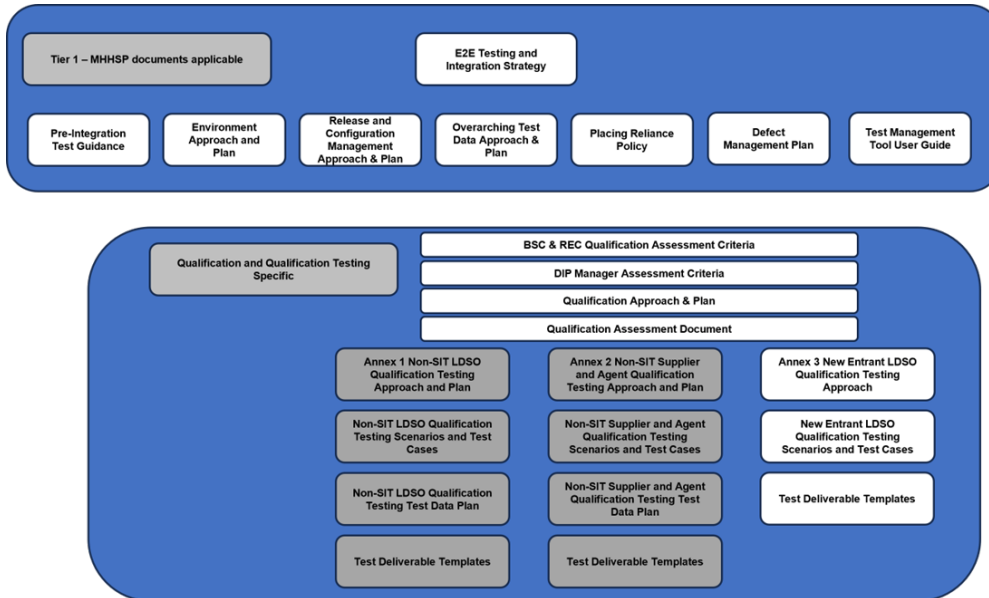
Figure 1: Document Hierarchy
